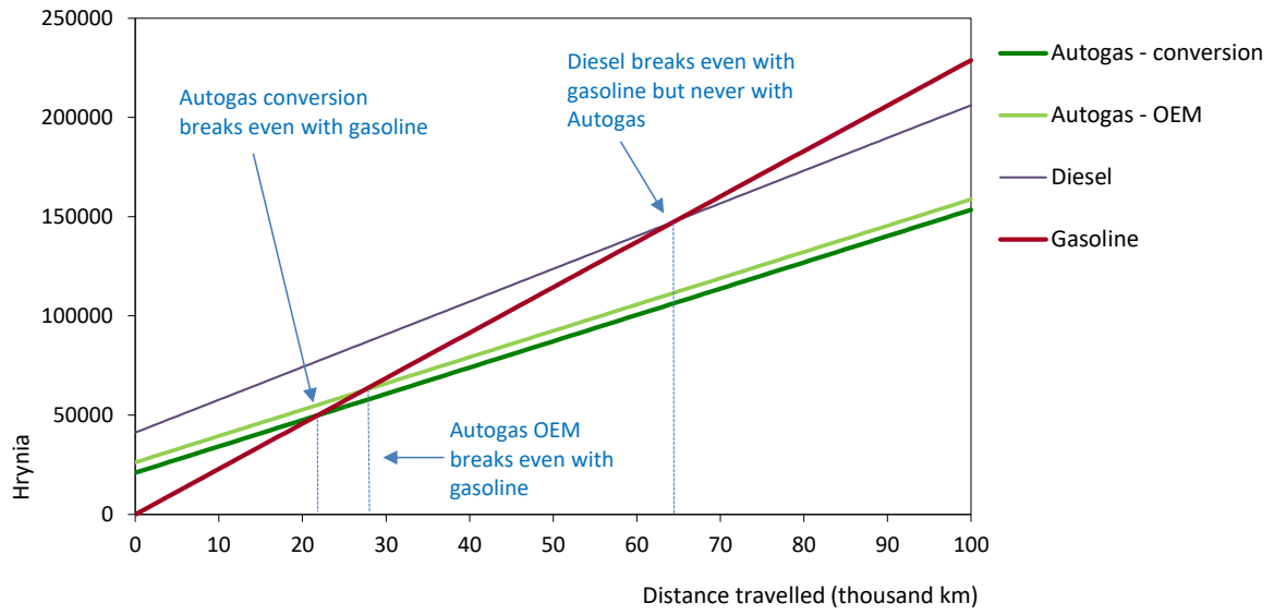
Figure B23.2: Running costs of a non-commercial LDV, 2018 – Ukraine
