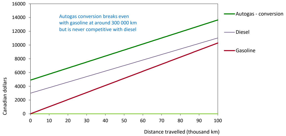
Figure B3.2: Running costs of a non-commercial LDV, 2018 – Canada
