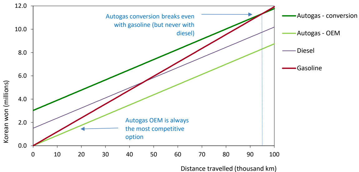
Figure B12.2: Running costs of a non-commercial LDV, 2018 – Korea
