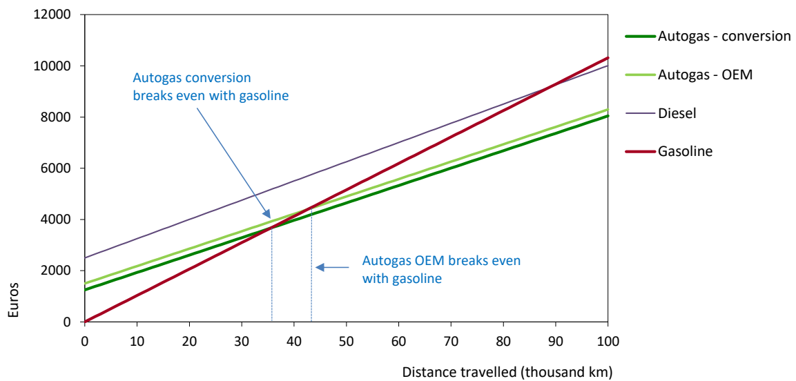
Figure B20.2: Running costs of a non-commercial LDV, 2018 – Spain
