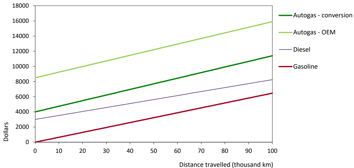
Figure B25.2: Running costs of a non-commercial LDV, 2018 – United States
