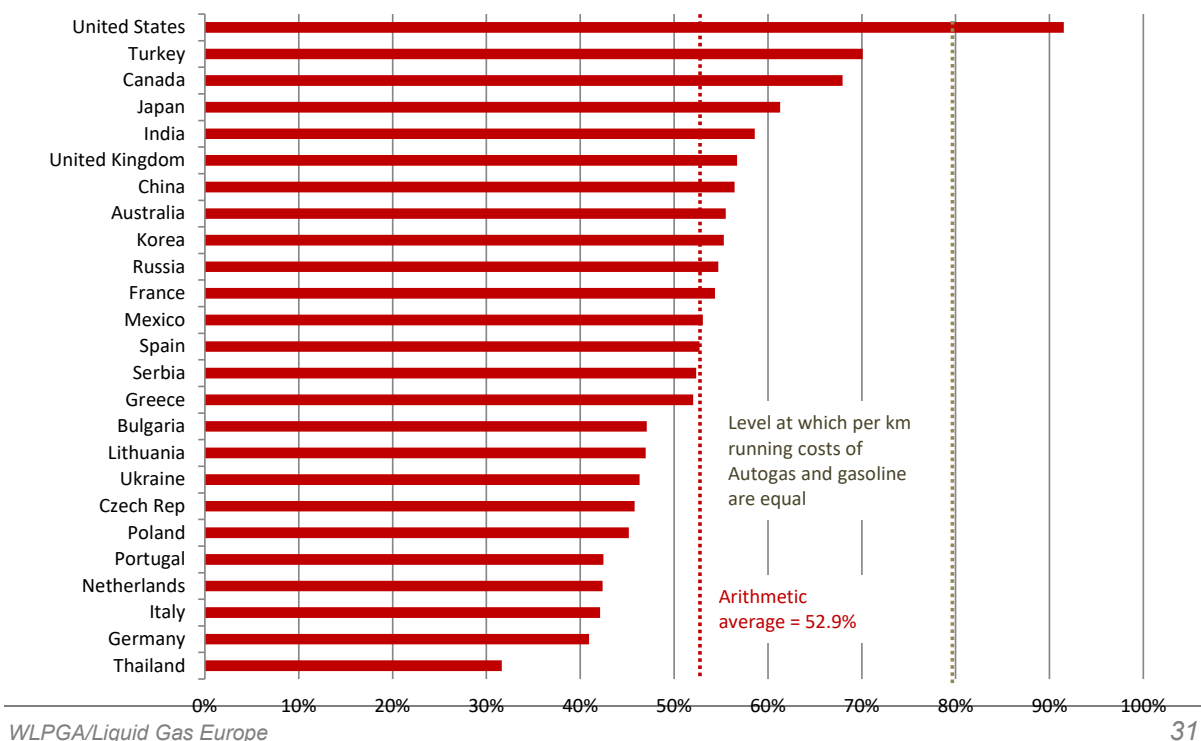
Figure A3.4: Autogas pump price including all taxes as % of gasoline price per litre, 2018
