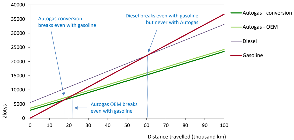
Figure B16.2: Running costs of a non-commercial LDV, 2018 – Poland
