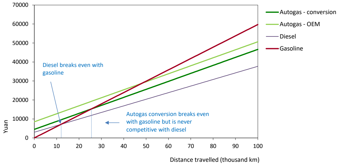
Figure B4.2: Running costs of a non-commercial LDV, 2018 – China
