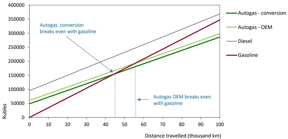
Figure B18.2: Running costs of a non-commercial LDV, 2018 – Russia
