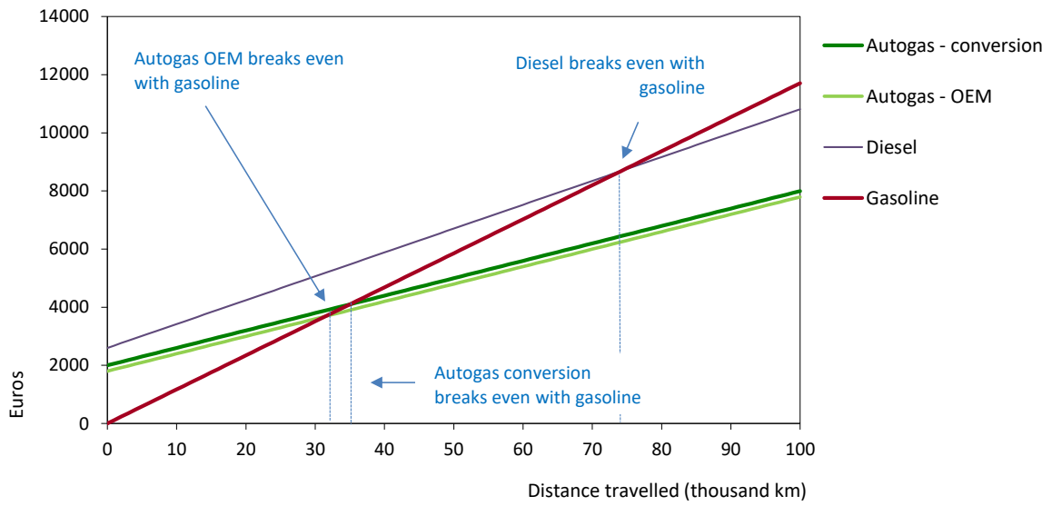
Figure B7.2: Running costs of a non-commercial LDV, 2018 – Germany
