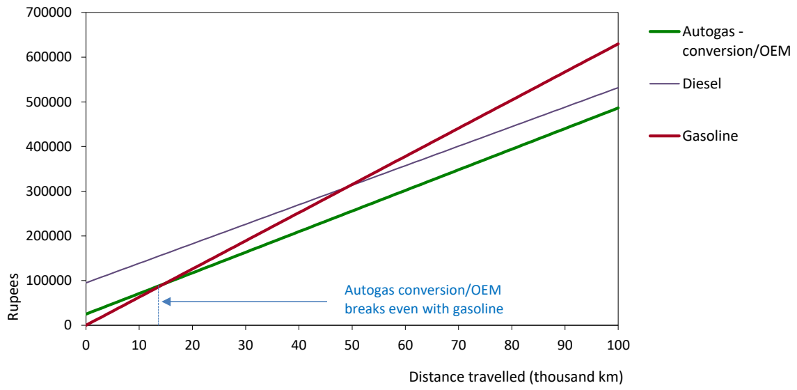
Figure B9.2: Running costs of a non-commercial LDV, 2018 – India
