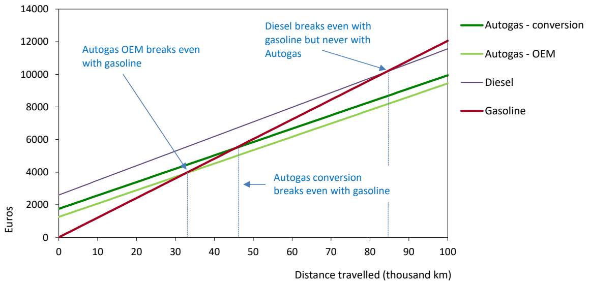
Figure B6.2: Running costs of a non-commercial LDV, 2018 – France
