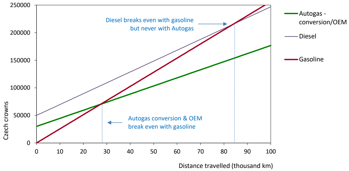
Figure B5.2: Running costs of a non-commercial LDV, 2018 – Czech Republic
