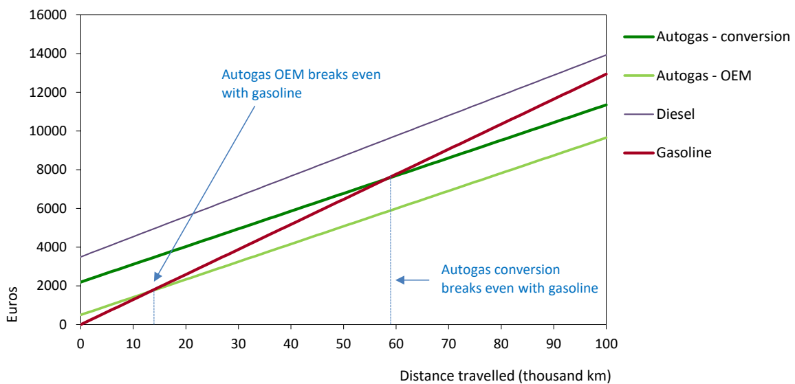
Figure B15.2: Running costs of a non-commercial LDV, 2018 – Netherlands
