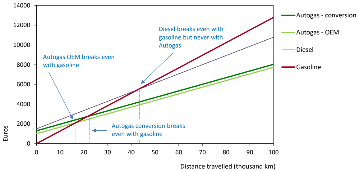
Figure B10.2: Running costs of a non-commercial LDV, 2018 – Italy
