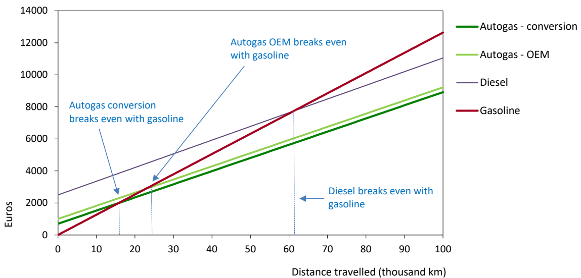
Figure B8.2: Running costs of a non-commercial LDV, 2018 – Greece
