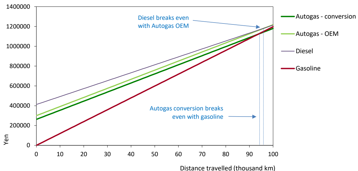
Figure B11.2: Running costs of a non-commercial LDV, 2018 – Japan
