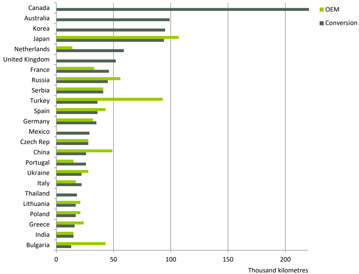
Figure A4.3: Autogas breakeven distance against gasoline, 2018
