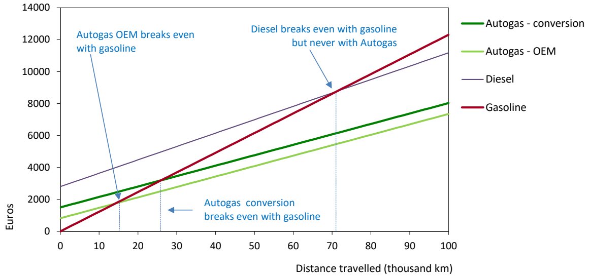
Figure B17.2: Running costs of a non-commercial LDV, 2018 – Portugal
