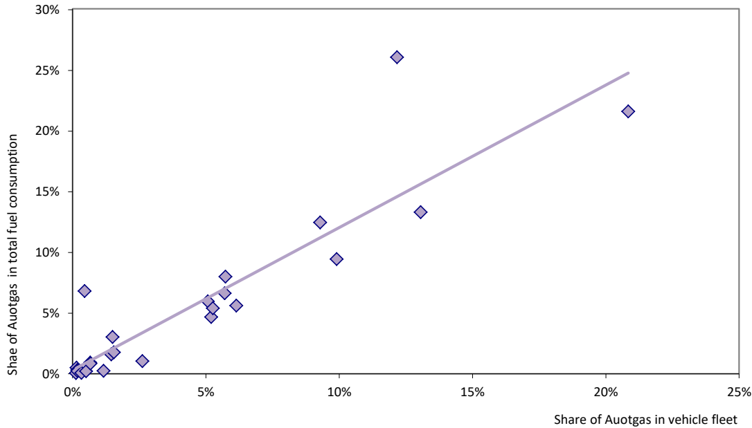
Figure A4.2: Share of Autogas in total automotive-fuel consumption versus vehicle fleet, 2017
