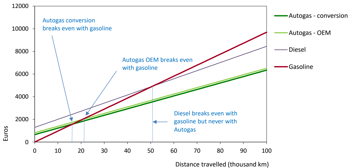
Figure B13.2: Running costs of a non-commercial LDV, 2018 – Lithuania
