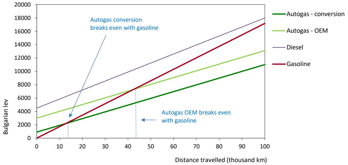
Figure B2.2: Running costs of a non-commercial LDV, 2018 – Bulgaria
