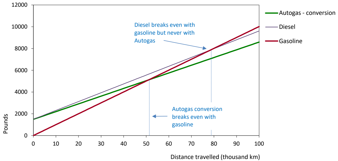
Figure B24.2: Running costs of a non-commercial LDV, 2018 – United Kingdom
