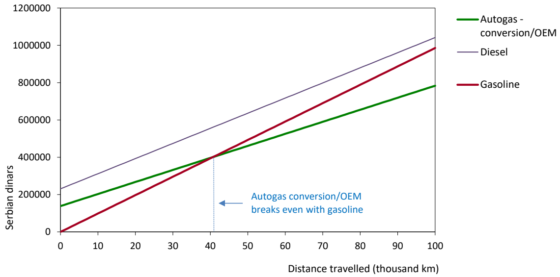
Figure B19.2: Running costs of a non-commercial LDV, 2018 – Serbia
