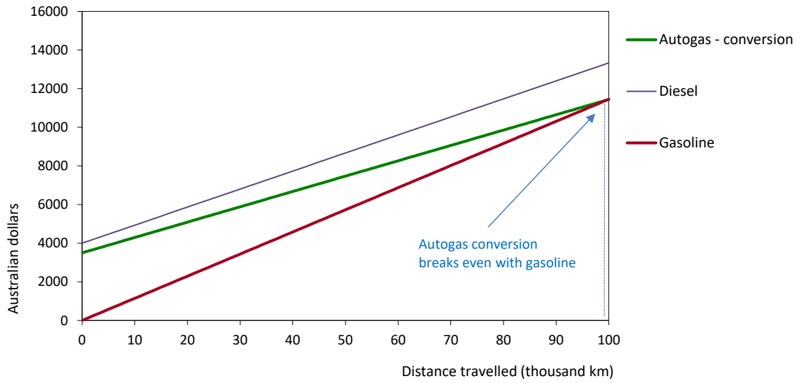
Figure B1.2: Running costs of a non-commercial LDV, 2018 – Australia
