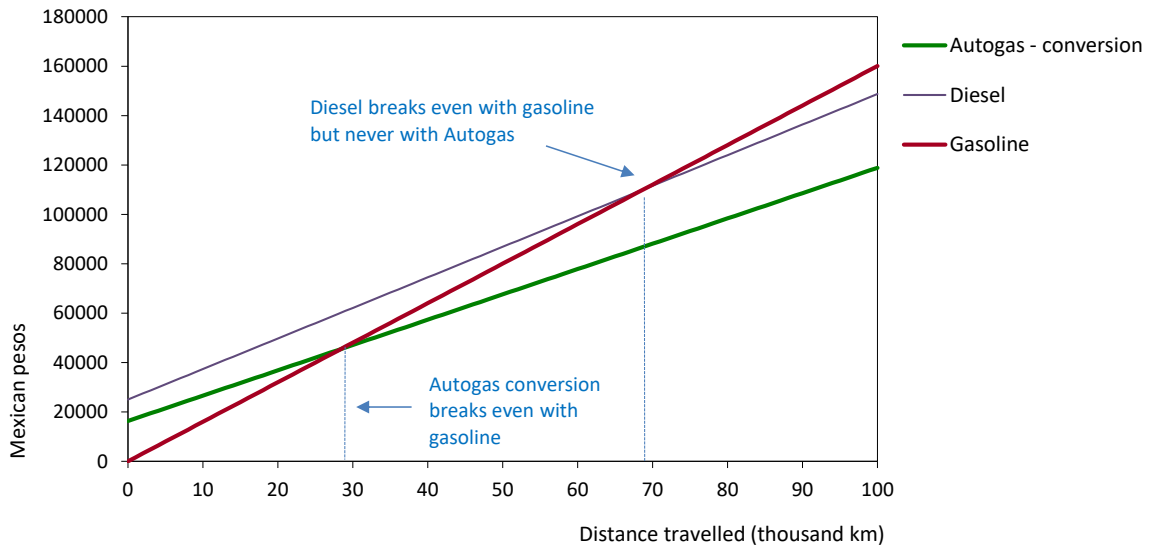
Figure B14.2: Running costs of a non-commercial LDV, 2018 – Mexico
