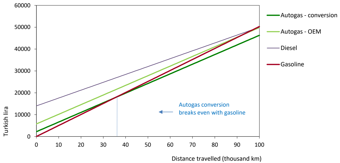
Figure B22.2: Running costs of a non-commercial LDV, 2018 – Turkey
