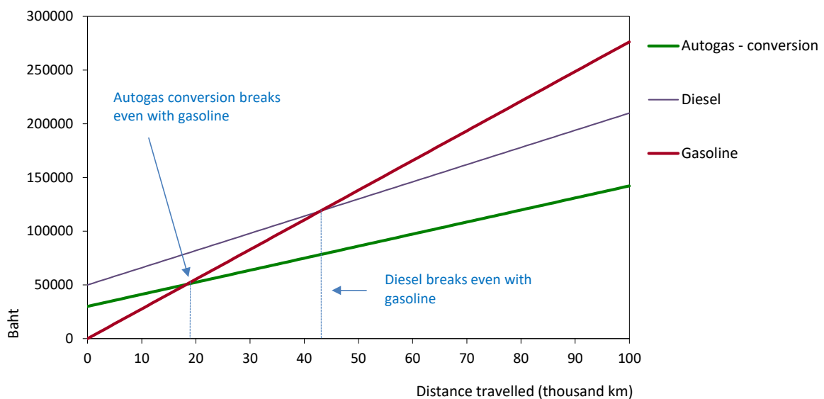
Figure B21.2: Running costs of a non-commercial LDV, 2017 – Thailand
